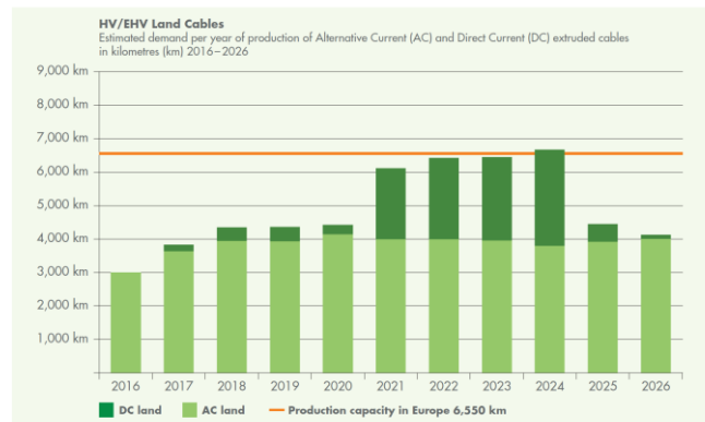
Europacable analysis of HV/EHV transmission cables demand in Europe 2016–2026 based on estimated year of production
